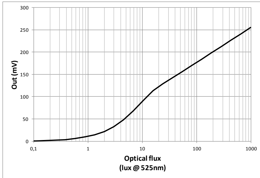
Fig. 6 NSC0902 sensor response
