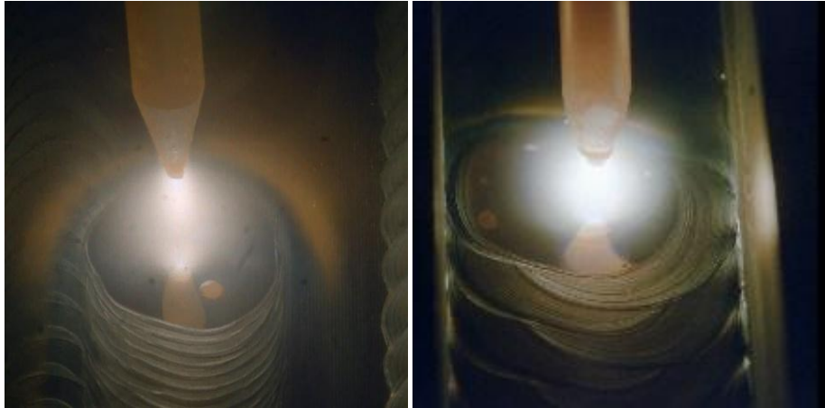
Fig.18 Images without (left) and with Filter
