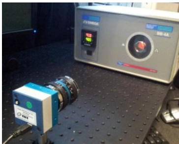
Fig.16 Widy SWIR 320U facing black body
