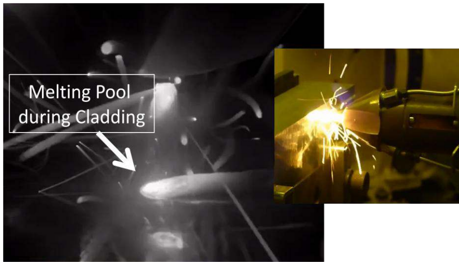
Fig. 14 Laser cladding imaging with NSC1003 Courtesy of Institut Maupertuis
