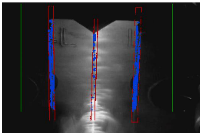
Fig.19 Weld view with post processing algorithm
