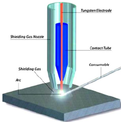
Fig.1 GTAW
