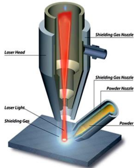
Fig.5 LAM principle
