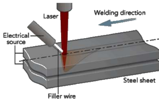
Fig .4 LBM principle
