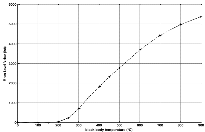
Fig.17 Widy SWIR response (DL count vs T°C)
