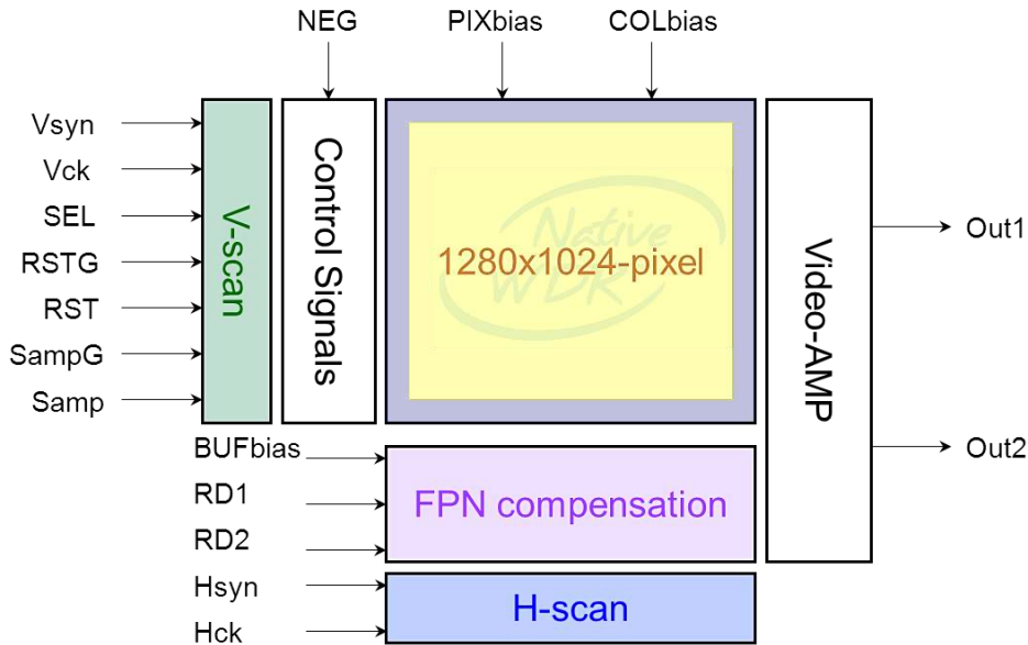
Fig.10 Function block diagram of NSC1003
