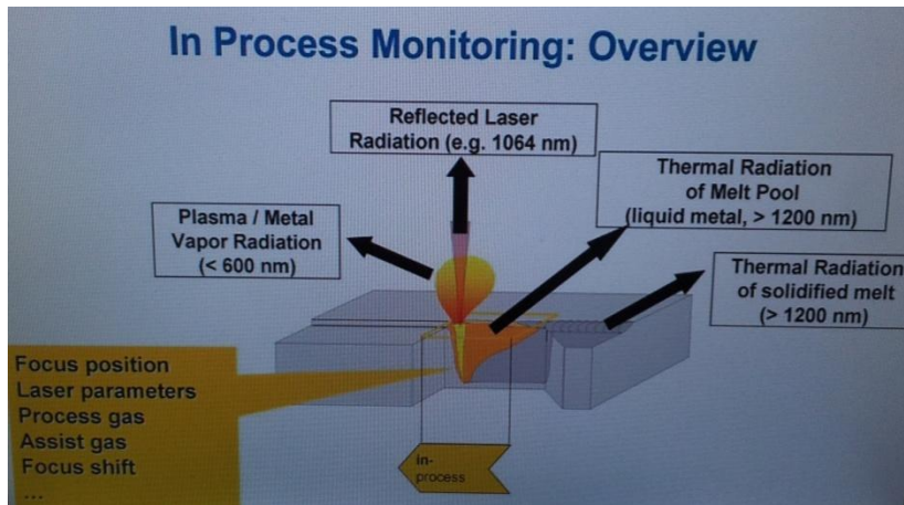
Fig. 15 Wavelength emission of different element during LBW
